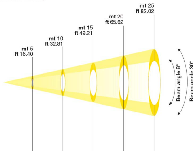
MSR Gold 700/2 Fastfit lamp
